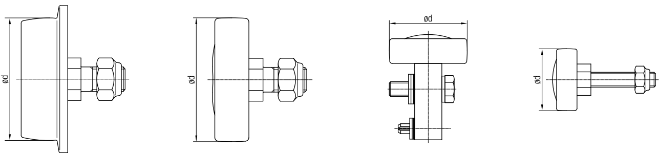
Flanged main roller Main roller cylindrical Horizontal guide roller Anti-lift roller
