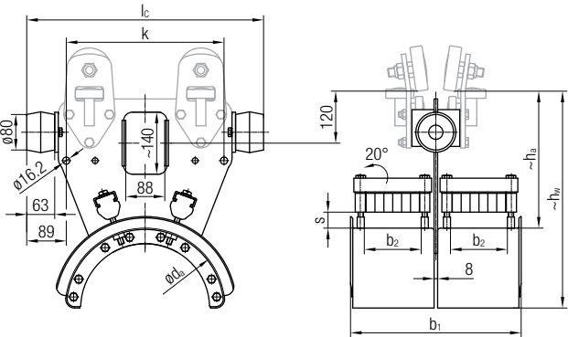
Towing trolley for catenary trolley
